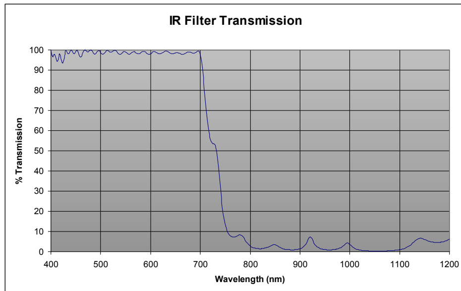
Typical Transmission of IR Filter
